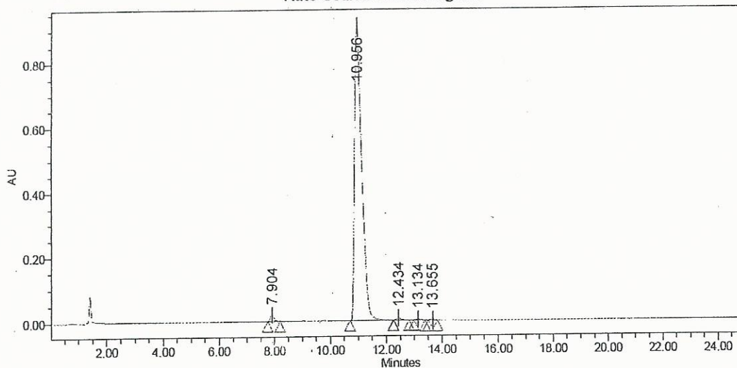
Auto-Scaled Chromatogram
